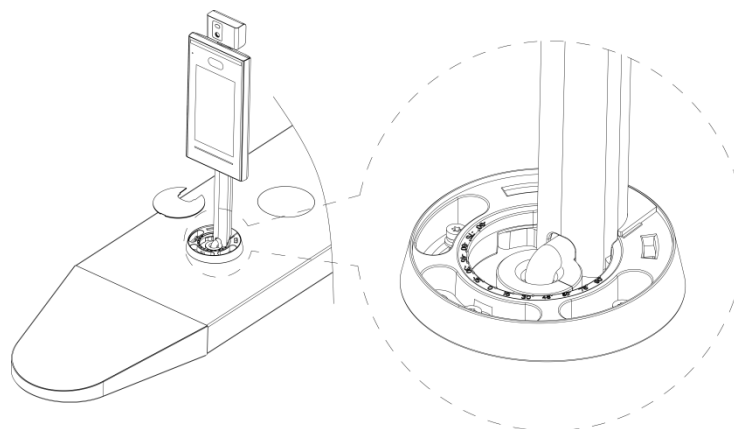
Figure 2-6 Applying silicon sealant to the terminal
